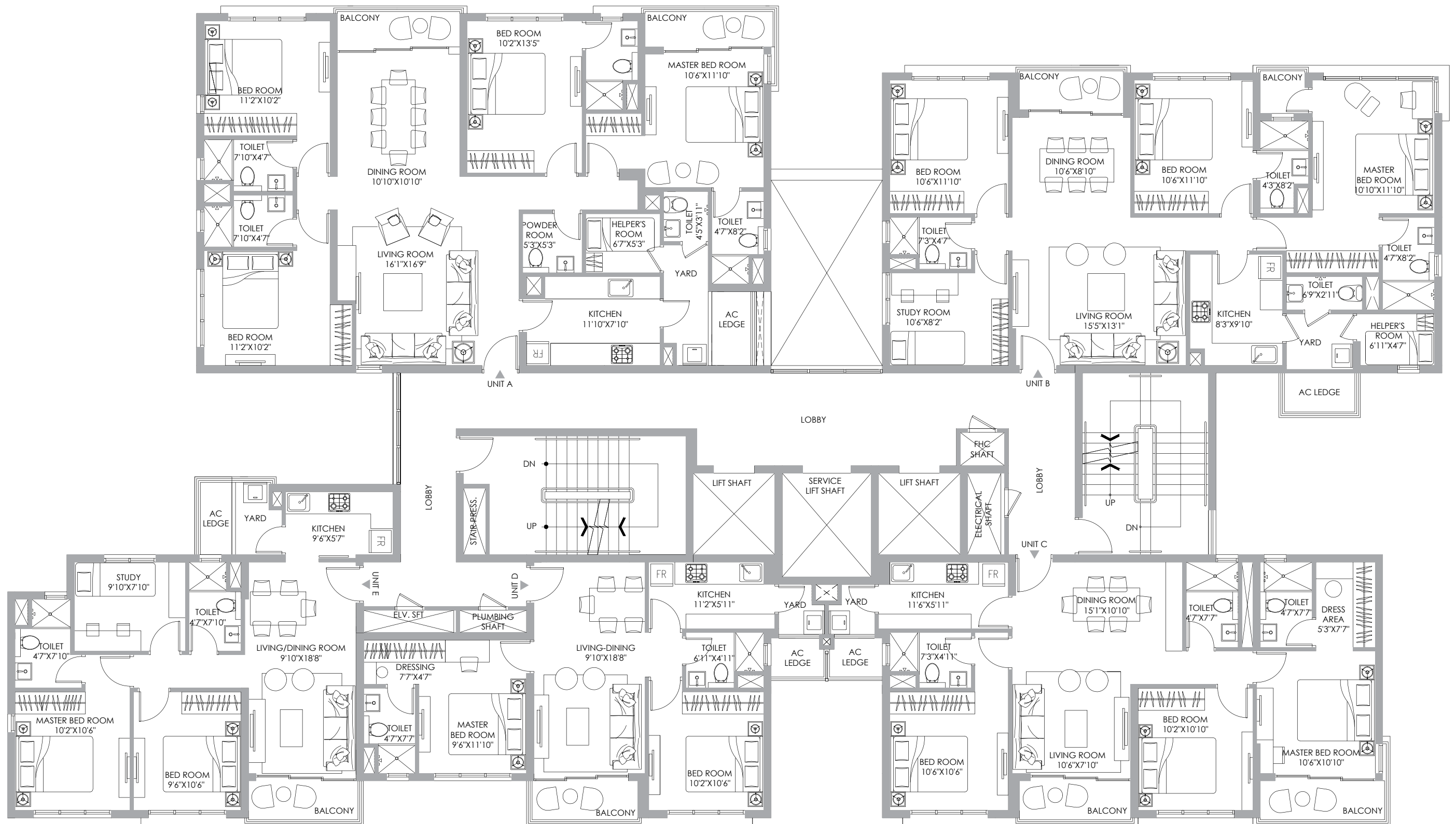
TYPICAL FLOOR PLAN: BLOCK 9
